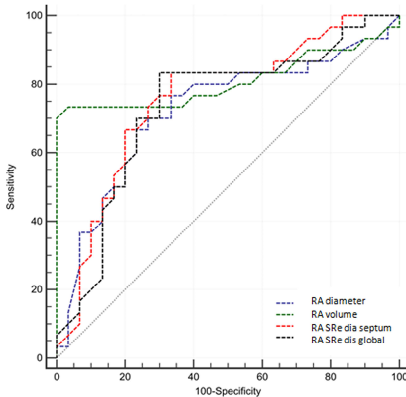
Figure 6. Receiver-operating characteristic (ROC) curves for discrimination between cases of inferior MI with or without RV involvement using RA diameter, RA volume, RA SRe dia septum or RA SRe dia global.
